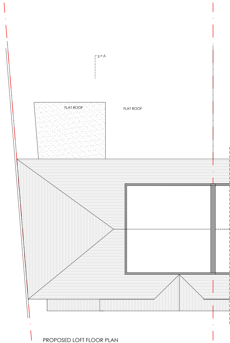
PROPOSED LOFT FLOOR PLAN
