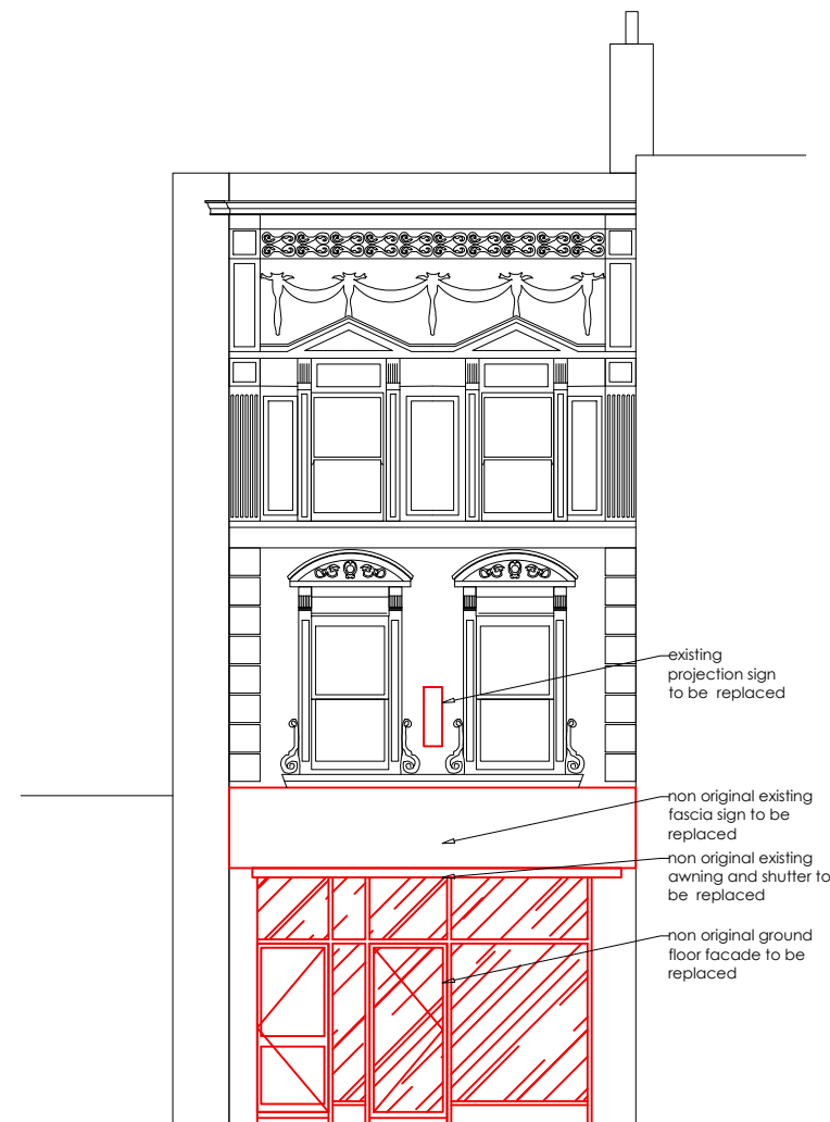
DEMOLITION FRONT ELEVATION
