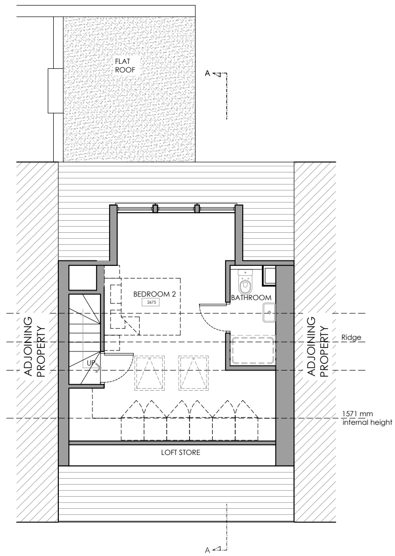
PROPOSED LOFT FLOOR PLAN
